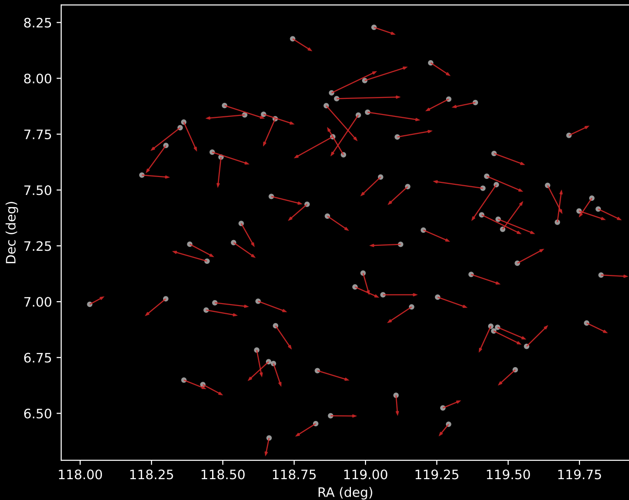
APOGEE DR17 Cluster 6 Proper Motion Vectors (n=80)
