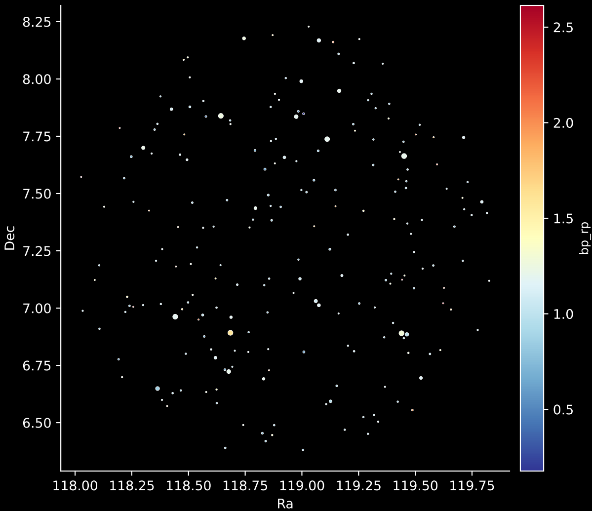
APOGEE DR17 Field: [133-55-O] Stars: 214
