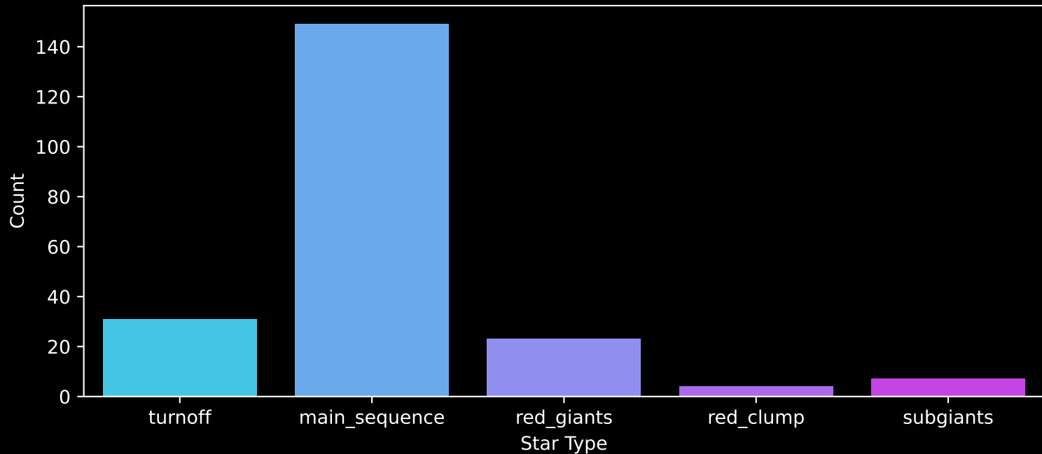
APOGEE DR17 Field: [133-55-O] Count plot of Star Type
