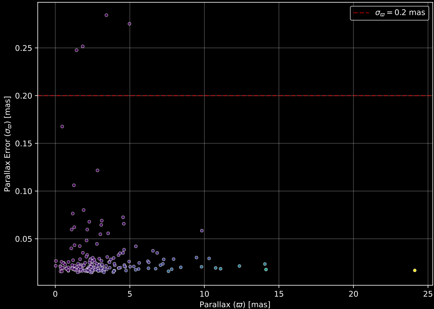
APOGEE DR17 Field: [133-55-O] Parallax Quality (n= 214)
