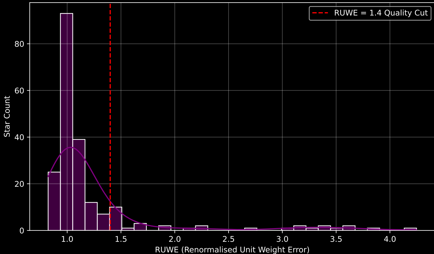
GAPOGEE DR17 Field [133-55-O] RUWE Distribution (n= 207)
