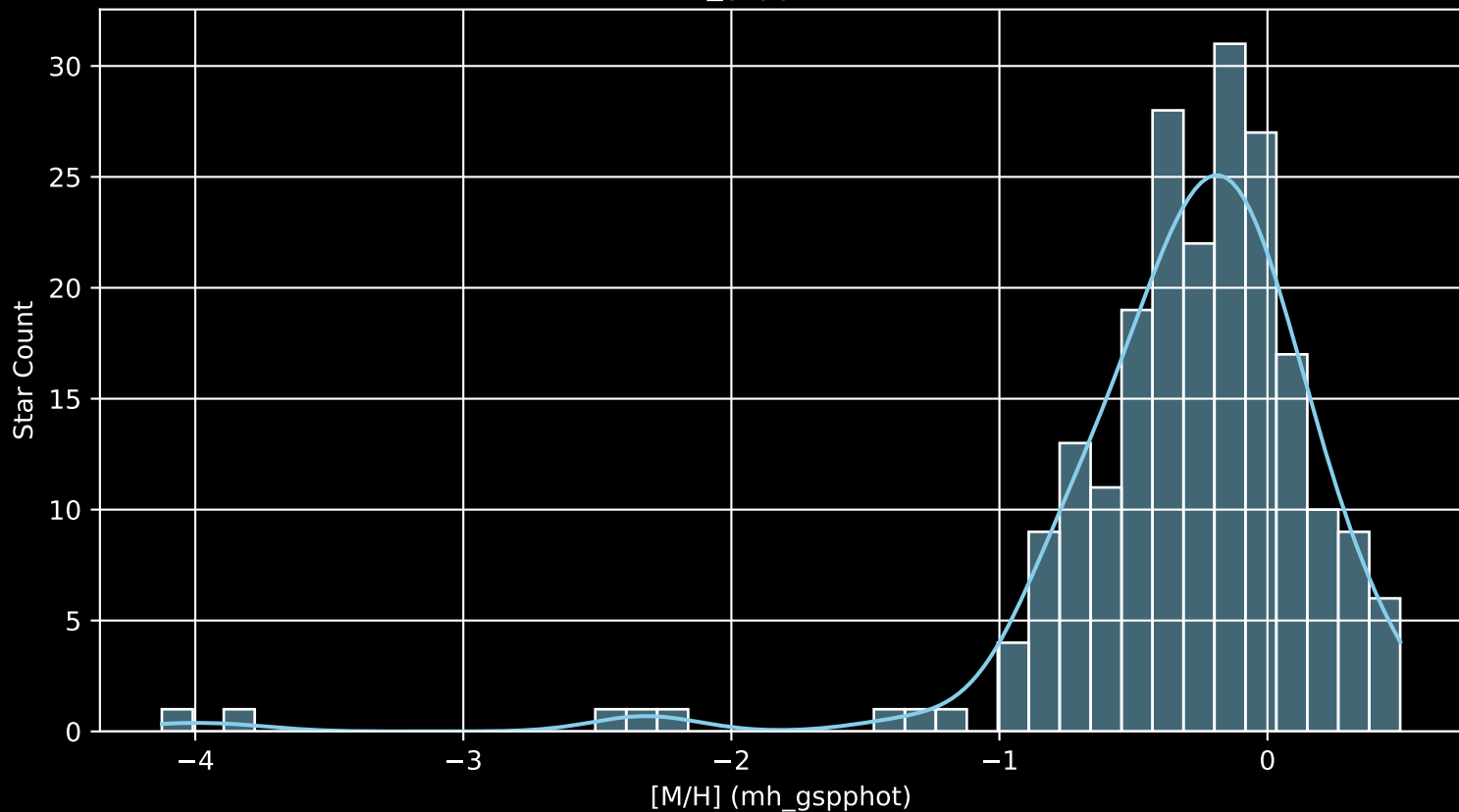
APOGEE DR17 Field: [133-55-O [M/H] (mh_gspphot) (n= 214)
