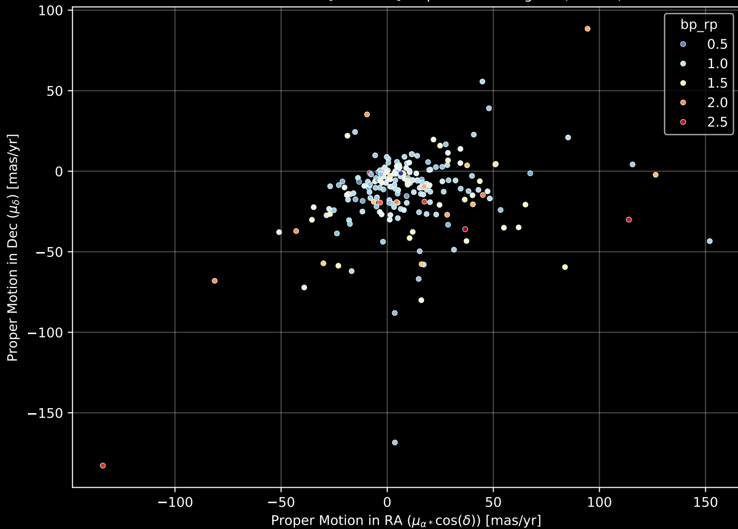
APOGEE DR17 Field: [133-55-O] Proper Motion Diagram (n= 214)
